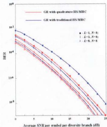
Figure 5. Comparison of the average BER of coherent BPSK and 8-PAM for GR with quadrature subbranch HS/MRC and HS/MRC schemes versus the average SNR per symbol per diversity for various values of 2L with N = 8 .
