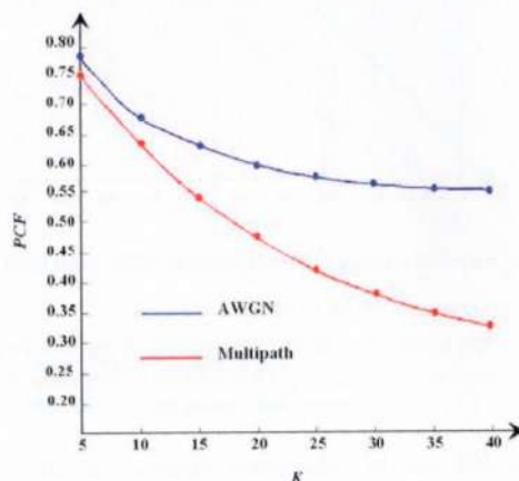
Figure 8. Optimal PCF versus the number of users: the AWGN and multipath channels.
