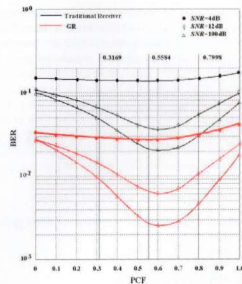
Figure 6. The BER performance of the single-stage GR based on PPIC with hard decisions for different SNRs and PCFs.
