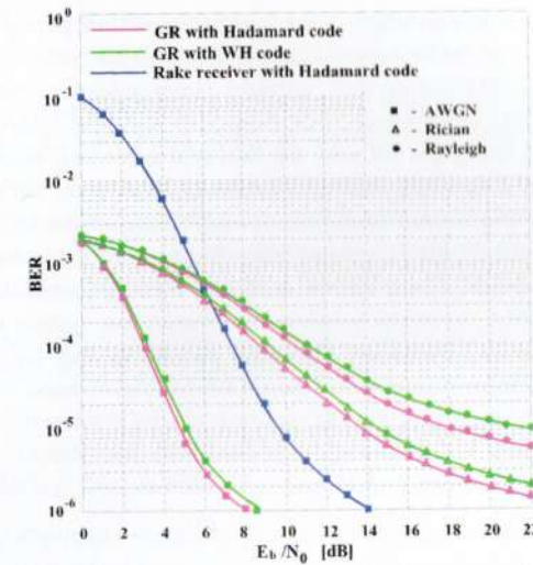
Figure 13. BER performance as a function of SNR E_b/N_0 in different channels ( K = 10, L = 4 ), MMRC.
