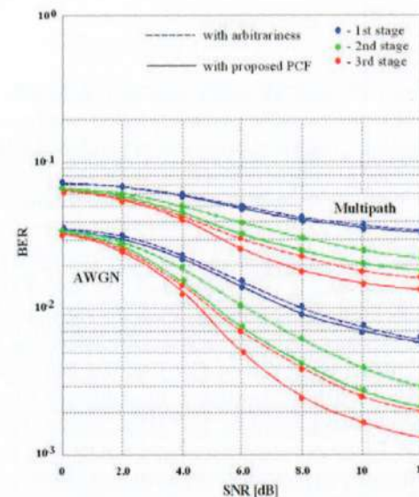
Figure 7. The BER performance at each stage for three-stage GR based on the PPIC with hard decisions for different PCFs at the first stage, i.e., the average value and an arbitrary value: AWGN and multipath channels.
