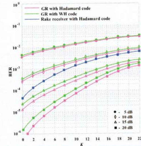
Figure 14. BER performance as a function of the number of users K . Rayleigh fading channel, MMRC, L = 4 .
