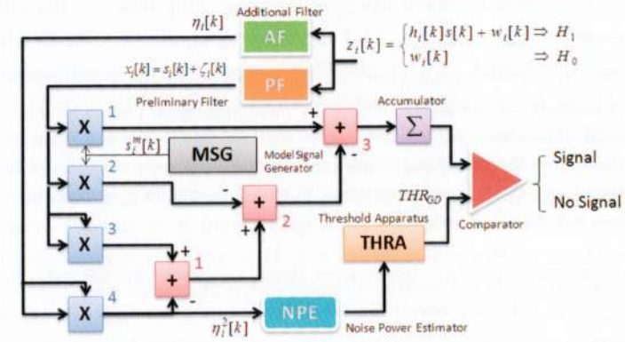
Figure 1. GR flowchart.
